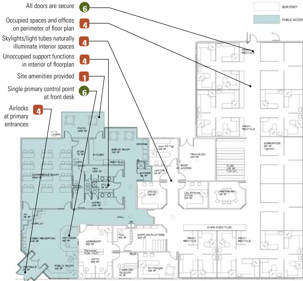
Preliminary Floor Plan - Fillmore Field Office, Utah
